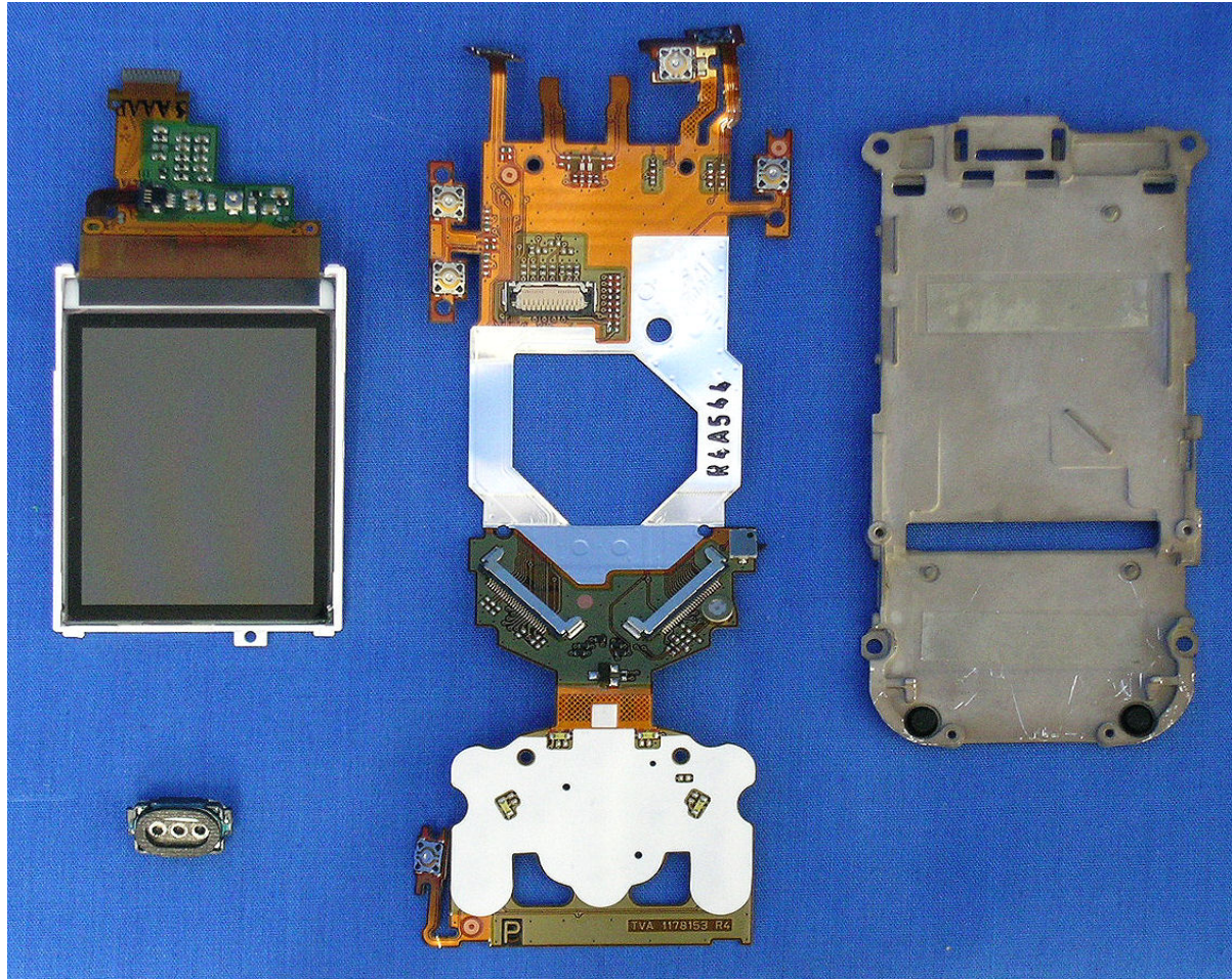
LCD Display, Flex Circuit and Support
