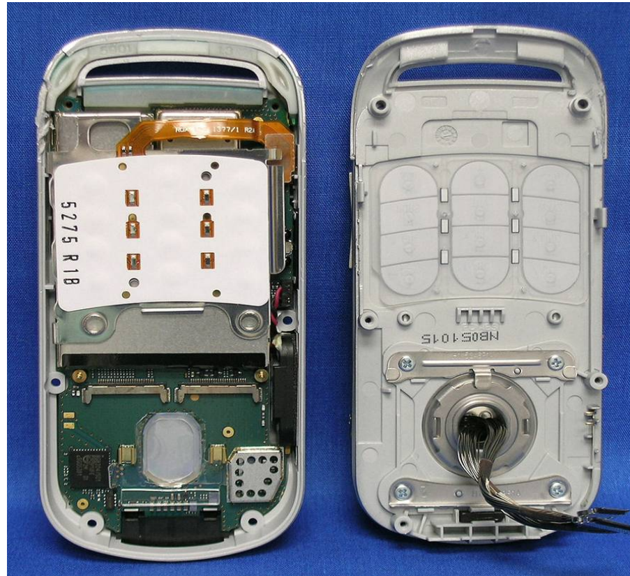
Rear Half Front Cover Removed
